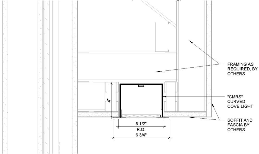
Section Detail A (direct fastening)
