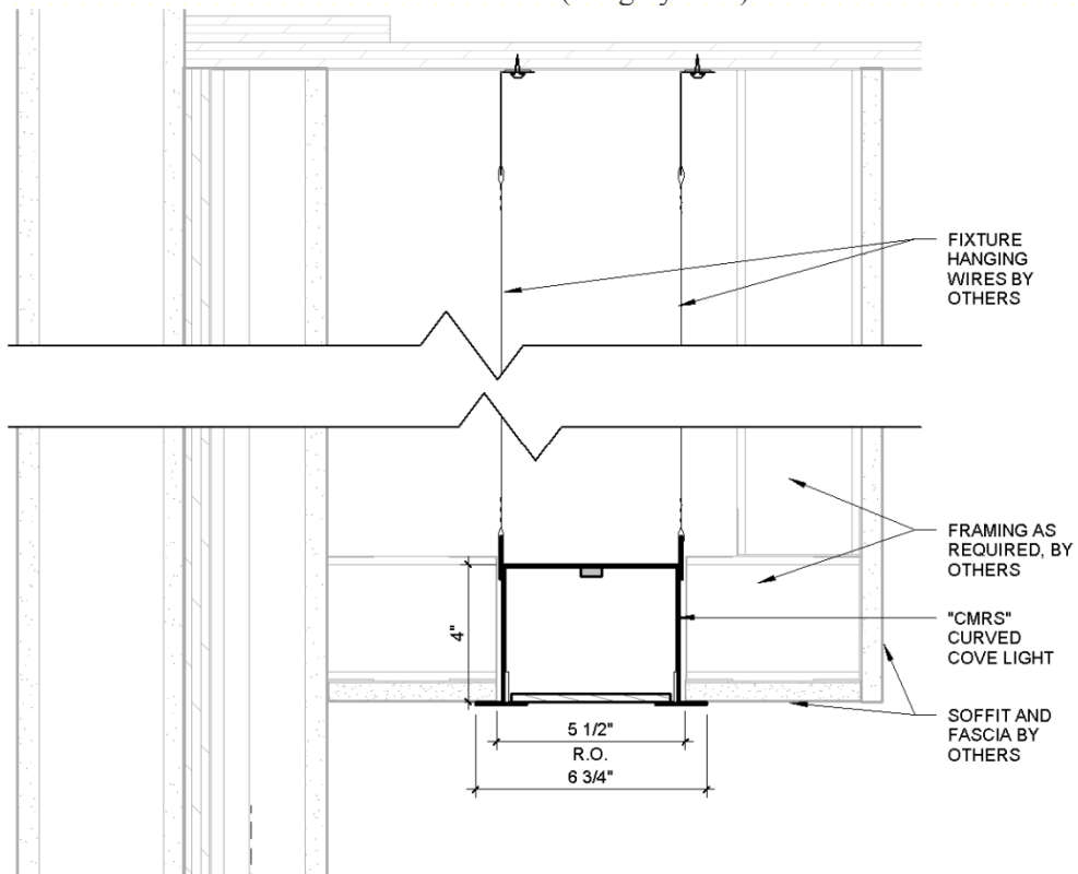
Section Detail B (hung by wire)
